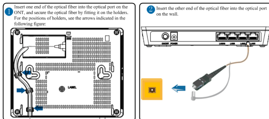
Figure 1-5 Optical ports on the HG8040H
