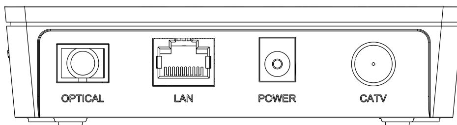
Figure 1-8 Ports and buttons on the rear panel of the HG8012H
