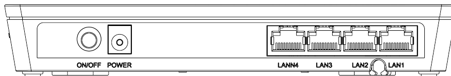
Figure 1-3 Ports and buttons on the rear panel of the HG8040H
